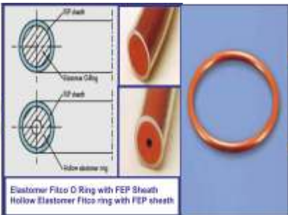
FEP O-Rings
